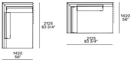
XL element
